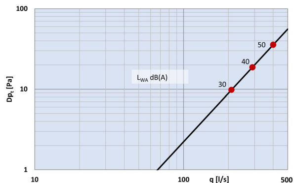
Diagram 5: Total A-weighted sound power level, dB(A) for SMID-250
