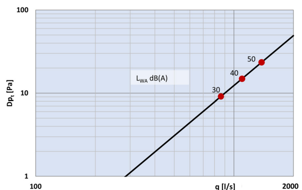
Diagram 8: Total A-weighted sound power level, dB(A) for SMID-500
