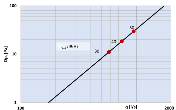
Diagram 7: Total A-weighted sound power level, dB(A) for SMID-400
