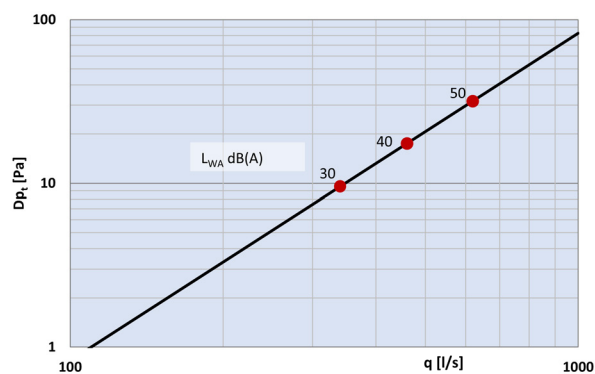
Diagram 6: Total A-weighted sound power level, dB(A) for SMID-315
