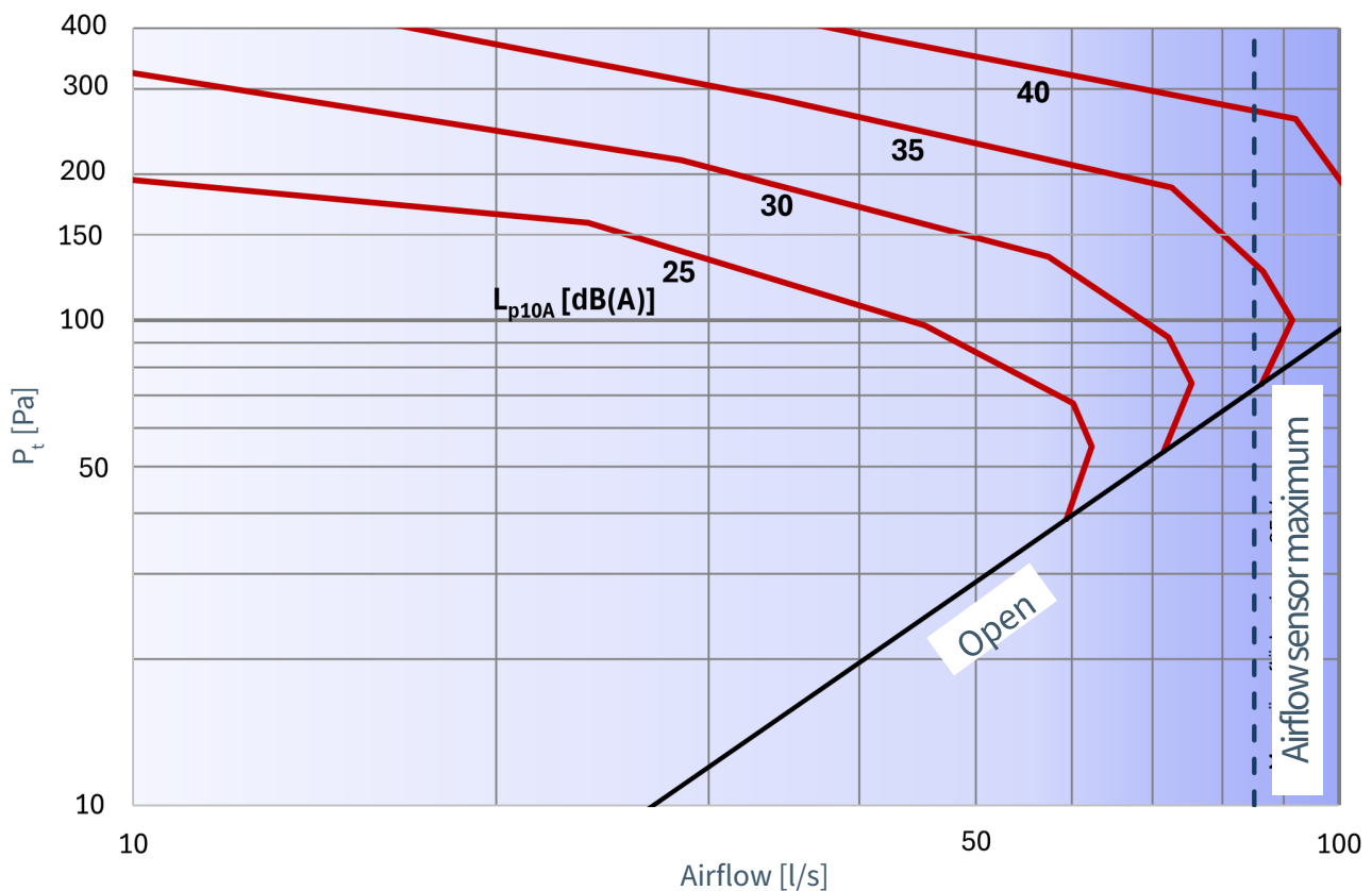
Diagram ISQ-V2, Sound pressure LPA dB(A)
