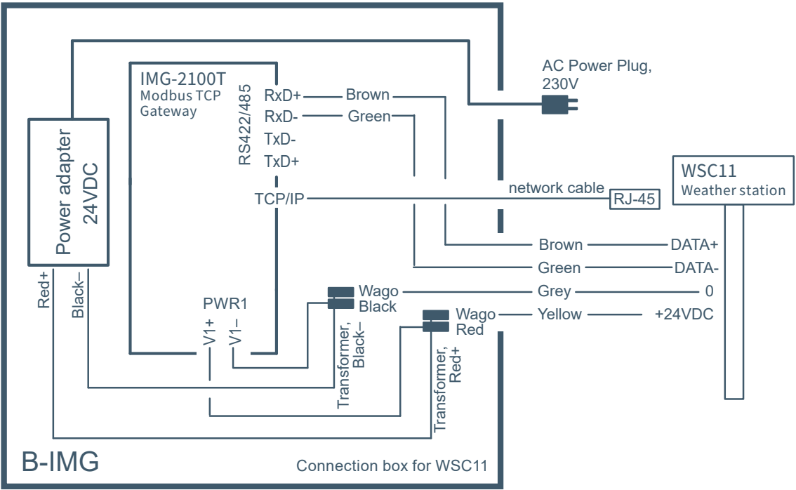
WSC11 with 5-core cable to EDW-100
