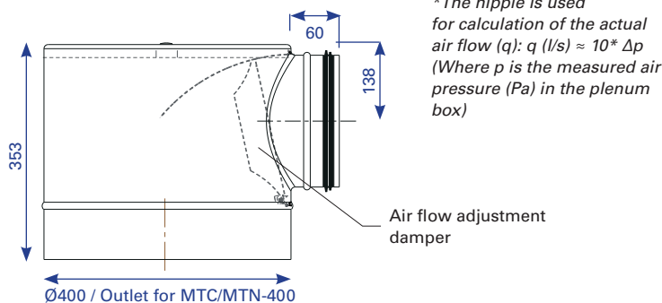
HMR-250/400: External dimensions in mm.
