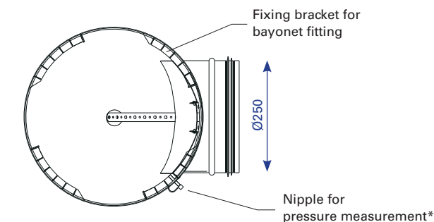
HMR-250/400: View from below; duct connection 250.
