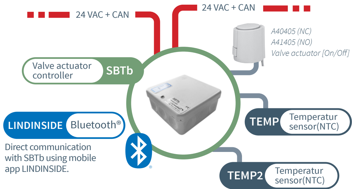
Connection diagram for SBTb. Actuators and temperature sensors are normally accessories that are ordered separately.
