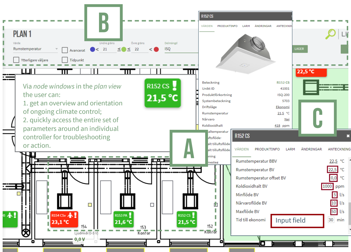
Part of the plan view with examples of node windows showing the current operating mode and a list of available values.
